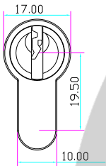
One side with cylinder the other side with thumbturn(factory default)
